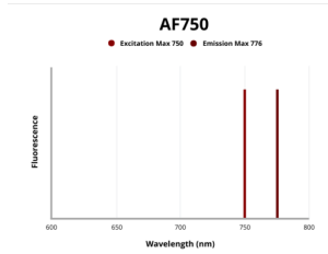
Fluorescence emission spectra of AF750.
