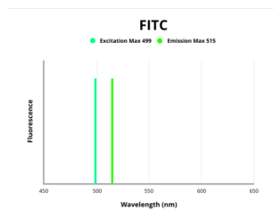
Fluorescence emission spectra of FITC.
