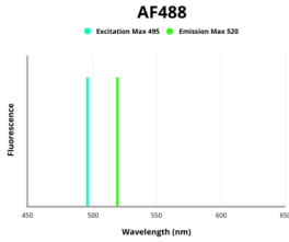
Fluorescence emission spectra of AF488.
