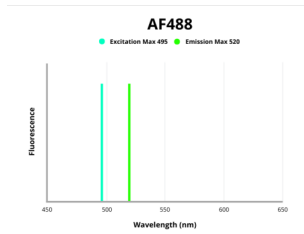
Fluorescence emission spectra of AF488.
