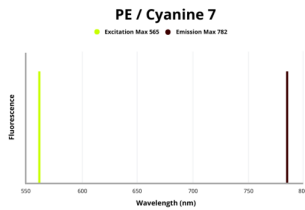
Fluorescence emission spectra of PE/Cyanine 7.
