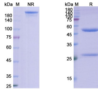
SDS-PAGE analysis of Ravagalimab in non-reducing (NR) and reducing (R) conditions.
