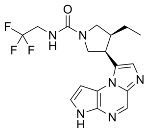
Chemical structure of Upadacitinib.
