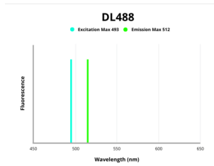
Fluorescence emission spectra of DL 488.
